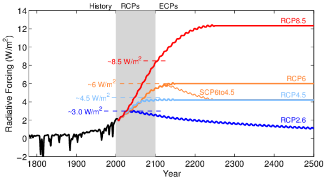
Box 1.2, Figure 1: Total radiative forcing (anthropogenic plus natural) for RCPs – supporting the original names of the four pathways as there is a close match between peaking, stabilization and 2100 levels for RCP2.6, RCP4.5 & RCP6, as well as RCP8.5, respectively. Note that the stated radiative forcing levels refer to the illustrative default median estimates only. There is substantial uncertainty in current and future radiative forcing levels. Short-term variations in radiative forcing are due to both volcanic forcings in the past (1800-2000) and cyclical solar forcing assuming a constant 11-year solar cycle (following the CMIP5 recommendation), except at times of stabilization (reproduced from Fig.4 in Meinshausen et al., 2011).
